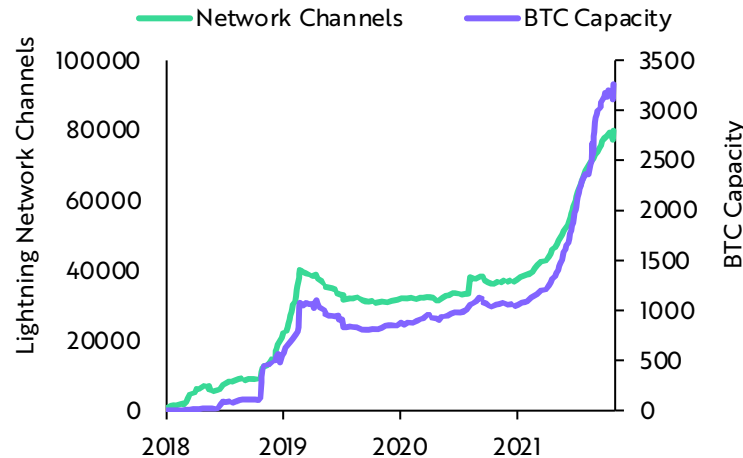
LN Channels and BTC Capacity*
